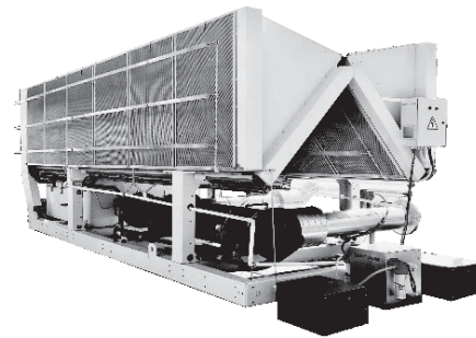
Chiller without Smart Cooling™ system
